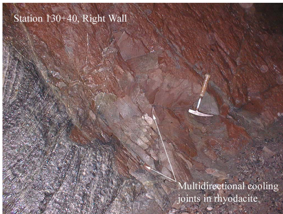
Figure 4 - Discordant intrusive contact of highly jointed rhyodacite (Dike # 3) that truncates metamorphic layering in the adjacent biotitized gneiss at a high angle. Note the multidirectional cooling joints both parallel to and crosscutting the contact with the gneiss and the thin, altered zone of contact metamorphism.
