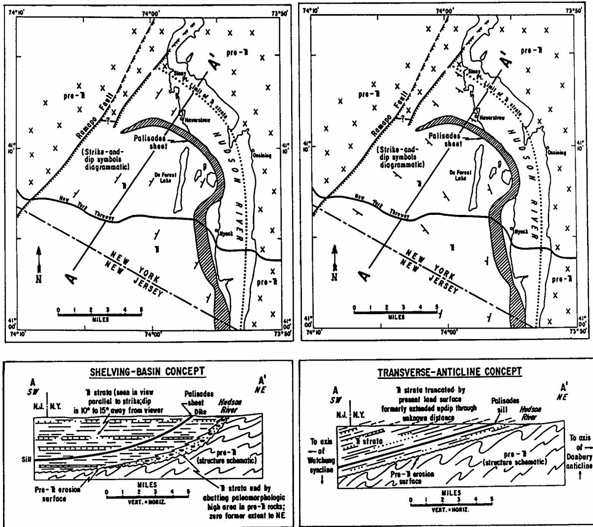
Figure 1. Schematic geologic maps of NE end of Newark basin in Rockland County, NY (above) and profile sections from Hudson River at Haverstraw to NY-NJ state line showing contrasting interpretations of the geologic relationships. (J. E. Sanders, 1974, figs. 7 and 8, p. 24-27; original artwork by staff of BP Alaska, New York office, courtesy John Conolly.)
