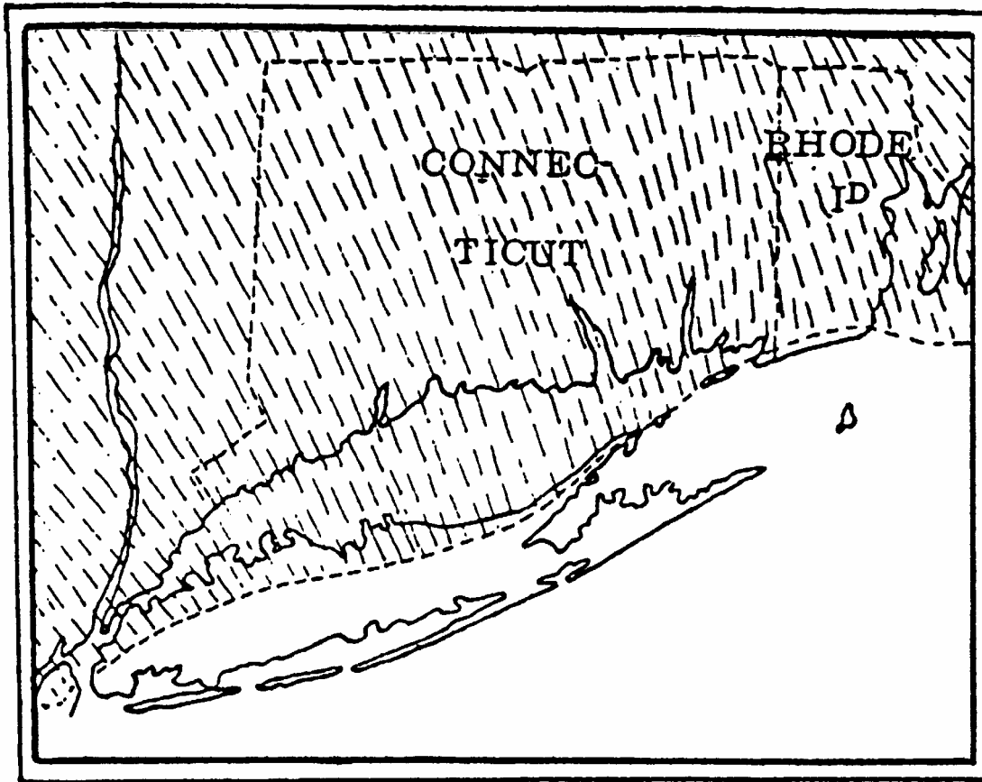
Figure 2. Sketch map of Connecticut, adjacent parts of New York, Rhode Island, and part of SE Massachusetts showing inferred regional SE-directed flow pattern in the glacier (No. II of our classification, Early Wisconsinan?) that deposited the Harbor Hill Moraine. (After J. H. Wilson, 1906, Plate II, fig. b, with N and E sides cropped.)
