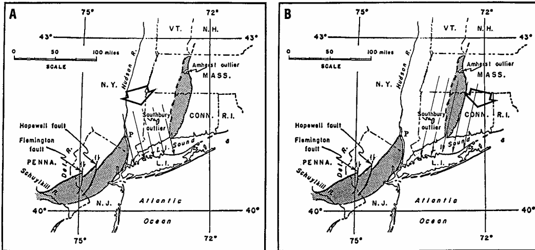
Figure 3. Regional sketch map of part of NE USA showing locations of preserved remnants of strata that filled Mesozoic nonmarine basins (Newark basin in NY, NJ, and PA; Hartford basin in CT and MA; light gray tone). Parallel line segments show how glacial ice flowing regionally from each of the observed dominant directions would distribute diagnostic erratics to Long Island. P = Peekskill, NY, near unique Cortlandt Complex of coarse ultramafic igneous rocks. (Base map from J. E. Sanders, 1963, fig. 7, p. 513.)
