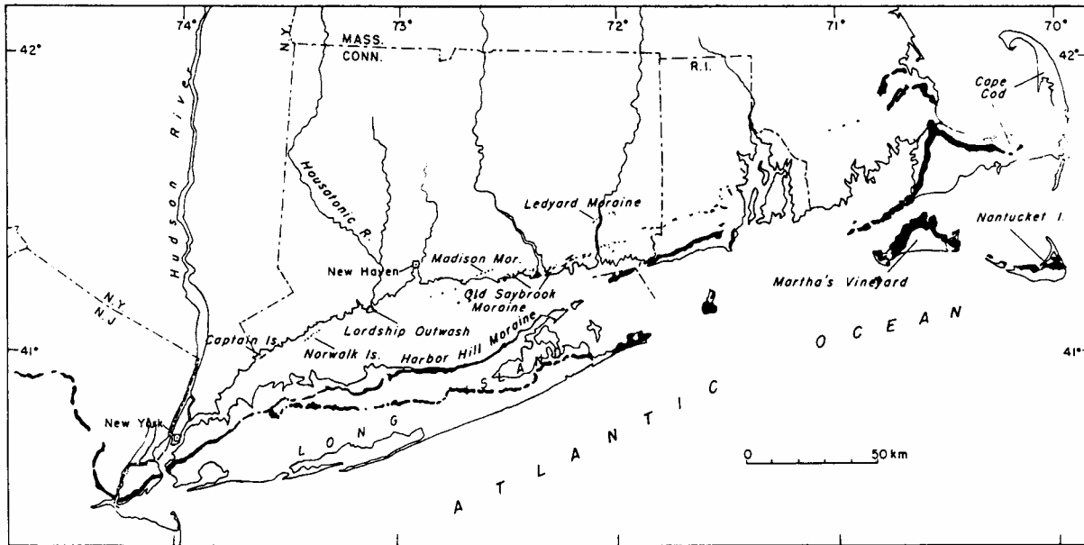
Figure 1. Sketch map of southern New England and vicinity, including adjacent islands showing locations of end-moraine ridges (black). We think that only the Old Saybrook and related moraines are products of the "Woodfordian" glacier that flowed from NNE to SSW. According to us, this moraine (of Glacier I in our proposed classification) was limited to coastal Connecticut as far W as the Norwalk Islands and extended southward so as to cross western Long Island (Queens and Brooklyn) only SW of these islands. (R. F. Flint and J. A. Gebert, 1974, fig. 4, p. 187.)
